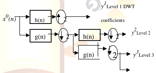
Fig.2 Filter bank representation of DWT decomposition:
